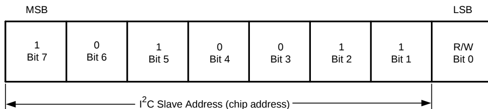
Figure 40. Device Address
