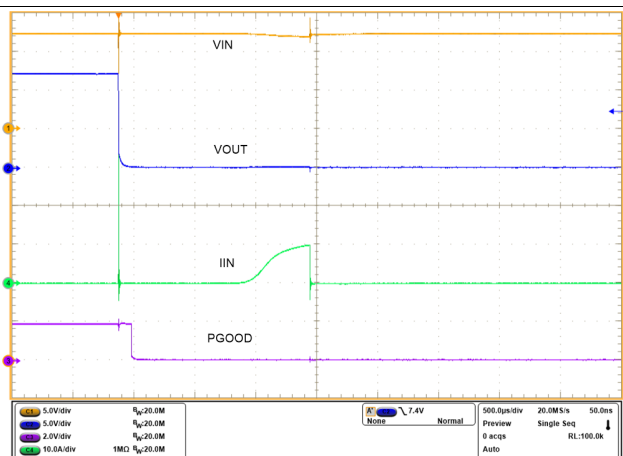
图 36. Circuit Breaker - Auto-Retry
