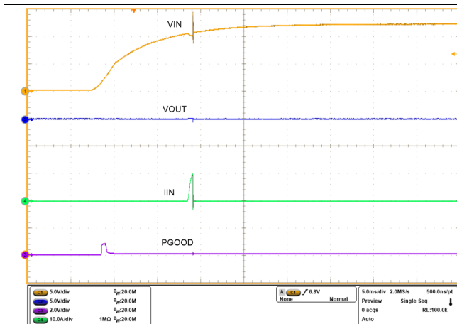
图 35. Circuit Breaker With Transient Overcurrent Blanking
