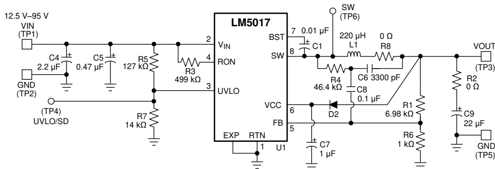
图 8-1. Final Schematic for 12.5-V to 95-V Input, and 10-V, 600-mA Output Buck Converter
