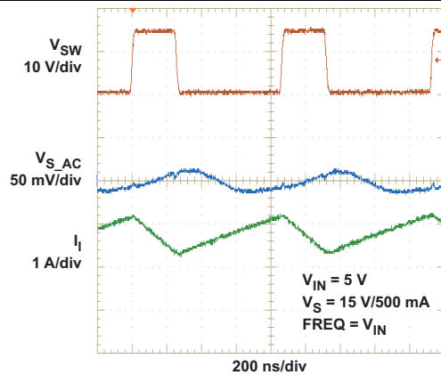
Figure 10. PWM Switching Continuous Conduction Mode
