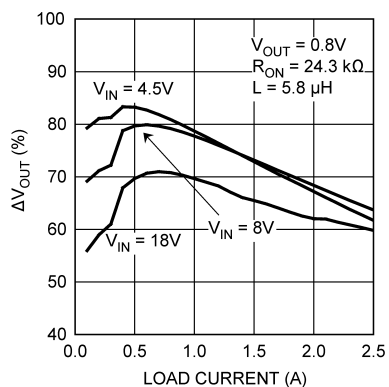
Figure 28. Efficiency vs Load Current ( V_{OUT} = 0.8\text{ V} )
