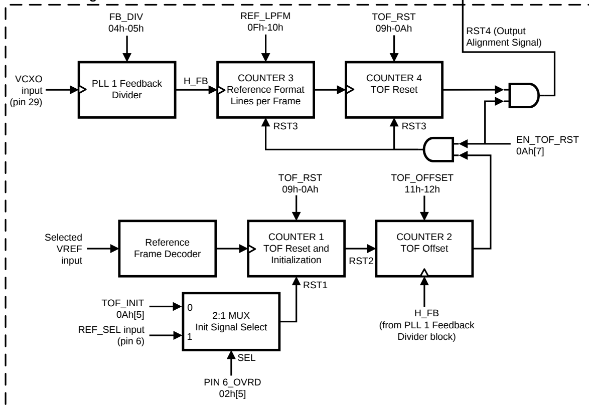
Figure 12. Functional Block Diagram – TOF Generation and Output Initialization Circuitry
