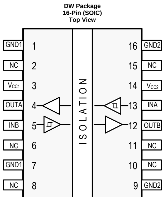
Pin Functions
