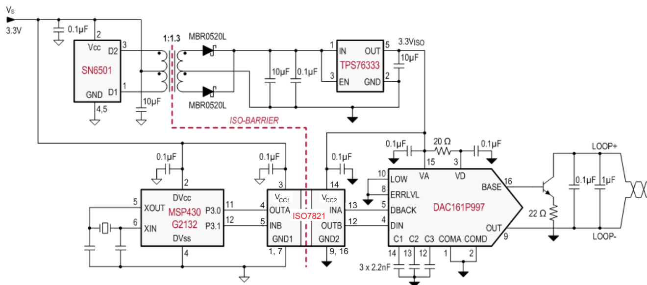
Figure 15. Isolated 4-20 mA Current Loop
