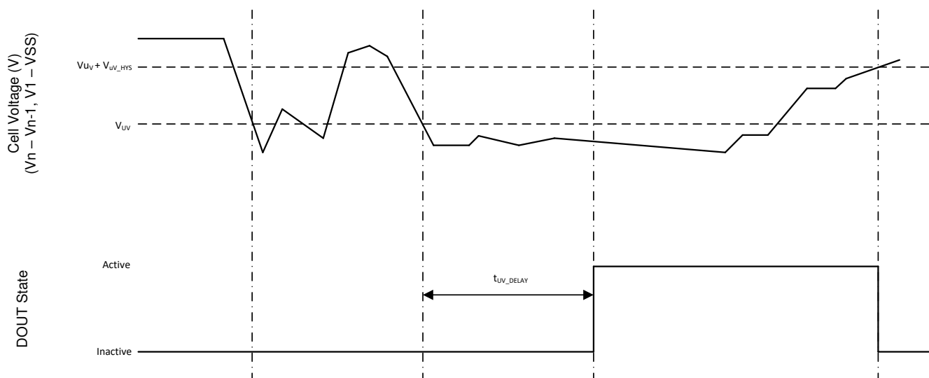
图 9-2. Timing for Undervoltage Sensing
