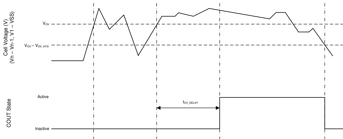
图 9-1. Timing for Overvoltage Sensing
