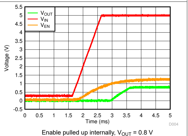
图 7-22. Startup With V_{EN} Floating
