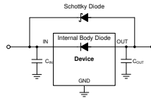
图 9-1. Example Circuit for Reverse Current Protection Using a Schottky Diode
