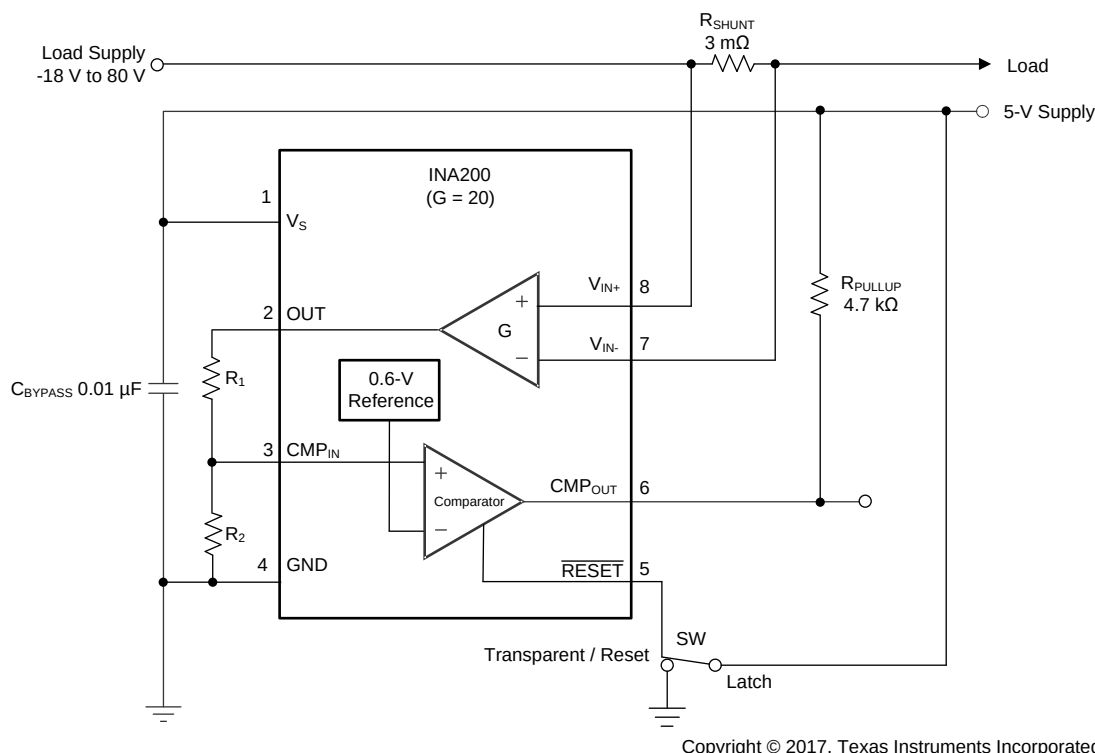
图 26. INA200 Basic Connections
