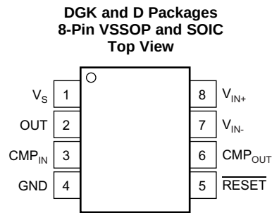
Pin Functions
