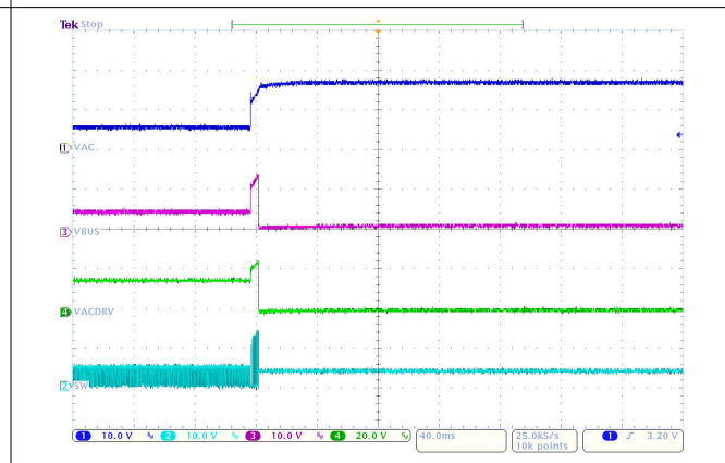
Figure 10-3. Power-Up with Charge Enabled
