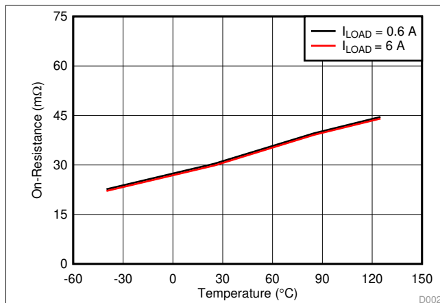
图 1. On-Resistance vs Temperature Across Load Current
