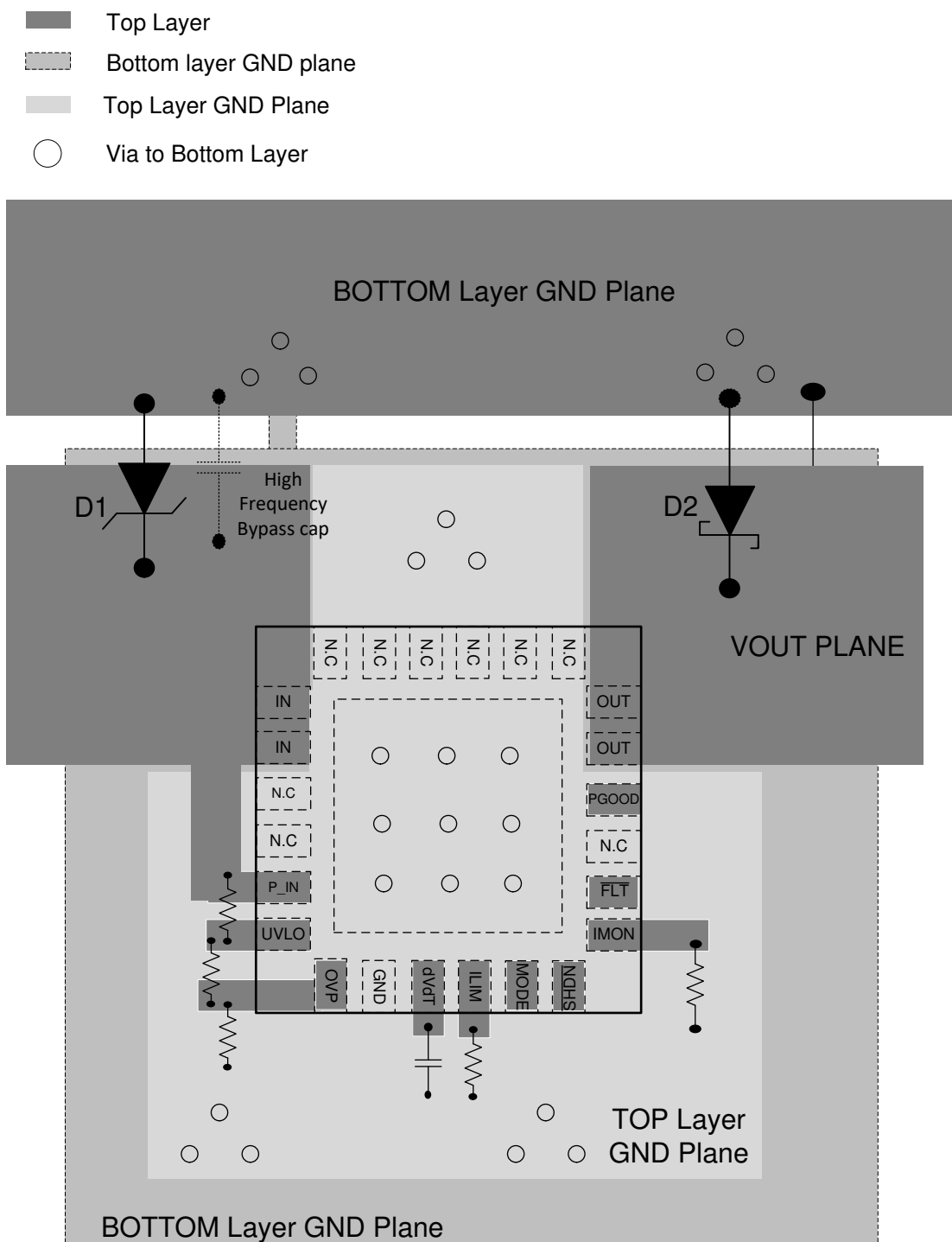
图 39. PCB Layout Example with QFN Package with a 2 Layer PCB
