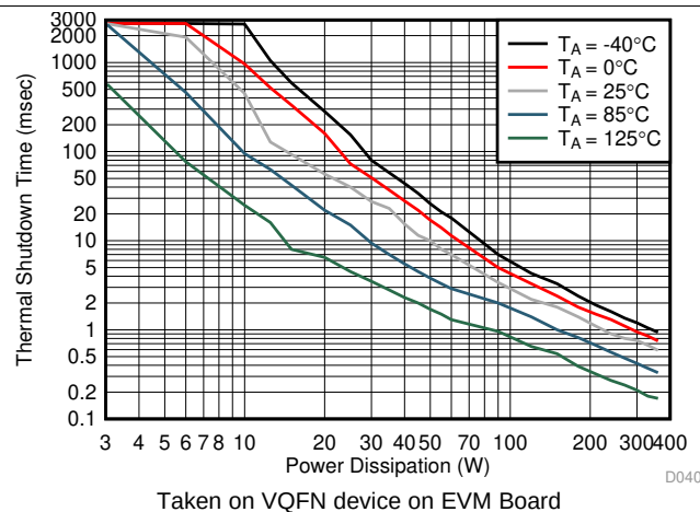
图 13. Thermal Shutdown Time vs Power Dissipation
