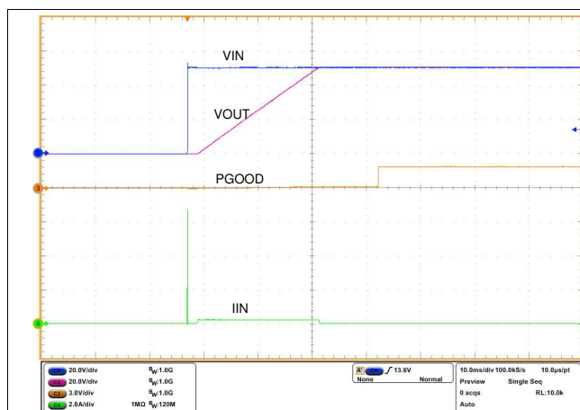
图 30. Hot-Plug In at 50-V Supply with No Load
