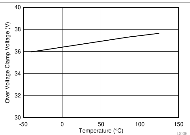
图 2. Overvoltage Clamp Threshold vs Temperature
