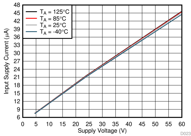
图 3. Input Supply Current vs Supply Voltage in Shutdown
