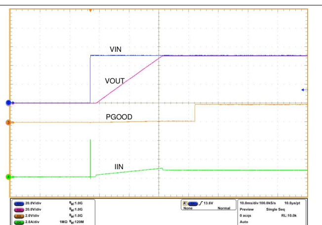
图 31. Hot-Plug In at 50-V Supply with 60- \Omega Load
