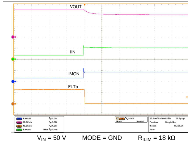
图 20. Overload Performance During Load Step from 140 \Omega to 40 \Omega
