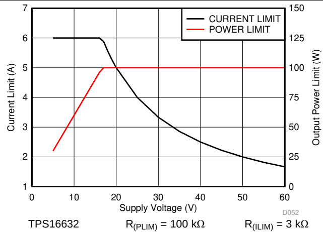
图 8. Power Limit, Current Limit vs Supply Voltage
