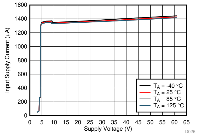
图 4. Input Supply Current vs Supply Voltage During Normal Operation
