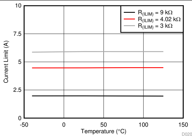
图 5. Overload Current Limit vs Temperature
