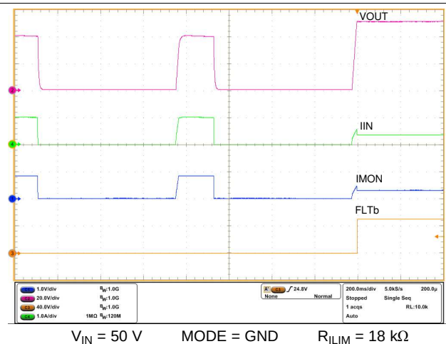
图 21. Coming Out of Overload with Load Step from 40 \Omega to 140 \Omega
