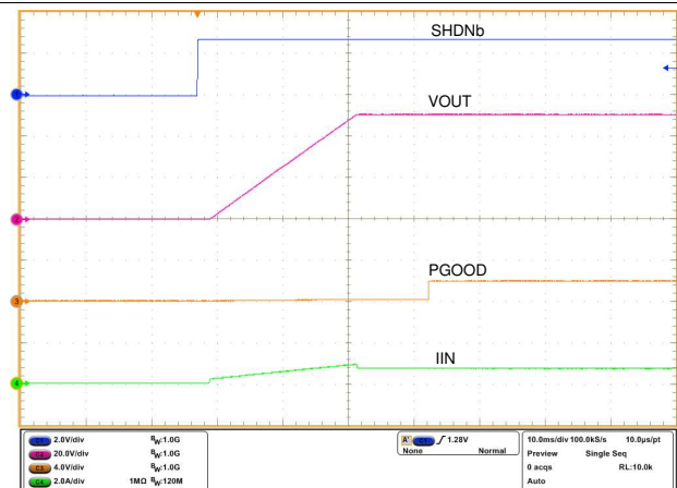
图 33. Coming Out of Overload with Load Step from 40 Ω to 140 Ω
