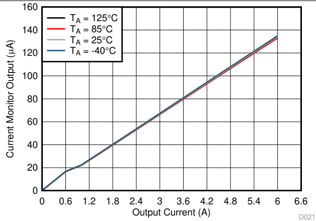
图 9. Current Monitor Output vs Output Current
