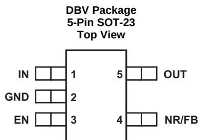
Pin Functions
