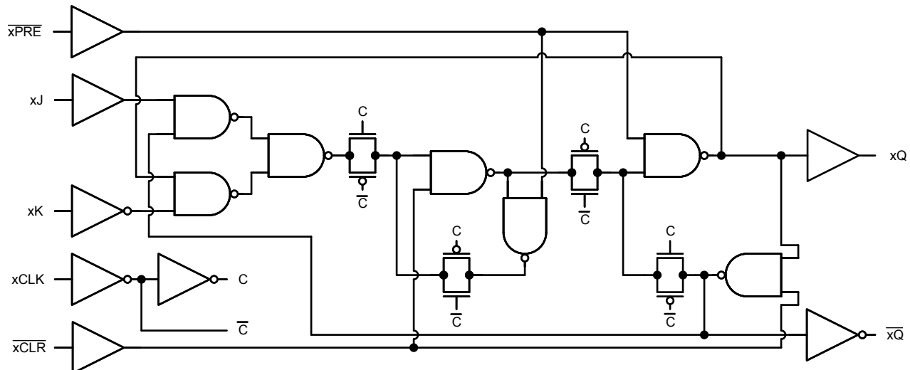
Functional Diagram
