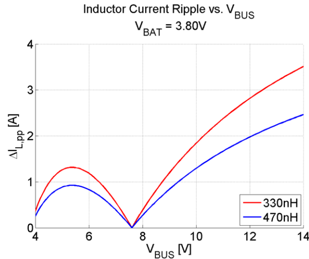
图 46. Inductor Current Ripple as function of V BUS with Fixed V BAT
