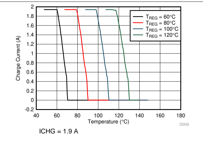
图 12. Charge Current vs Temperature
