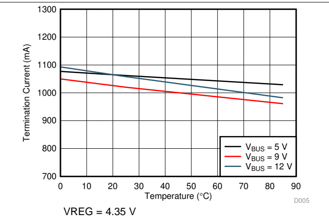
图 8. Termination Current vs Temperature
