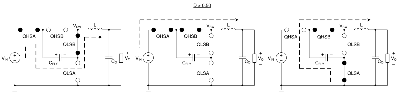
图 16. Three-Level Buck Converter States for Duty Ratios > 0.50
