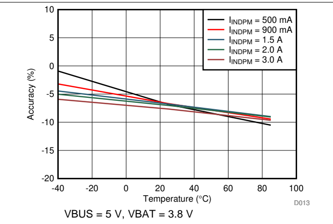
图 10. Input Current Limit Accuracy vs Temperature
