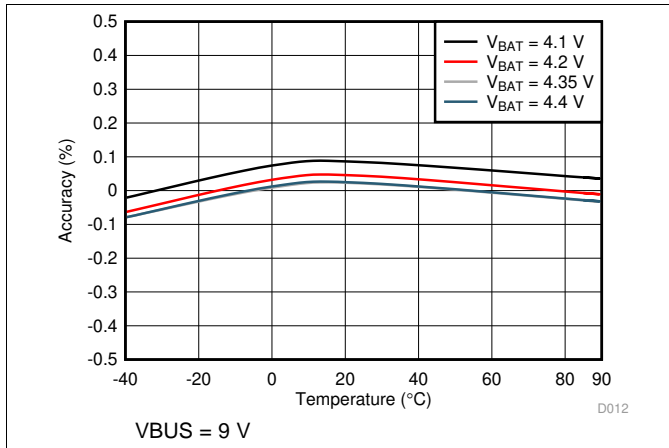
图 7. Battery Voltage Regulation Accuracy vs Temperature
