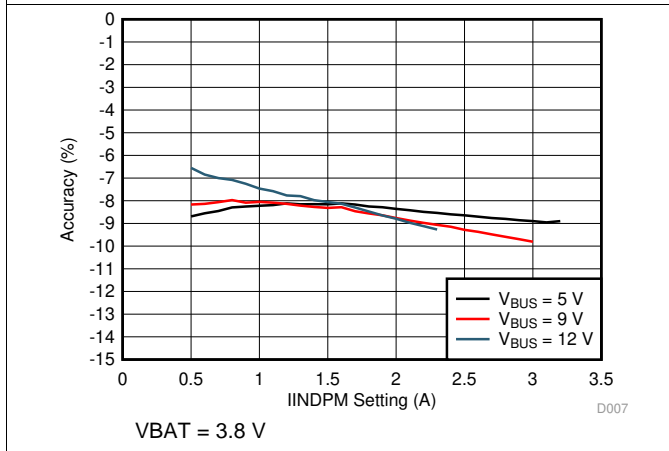
图 9. Input Current Limit Accuracy vs I 2 C IINDPM Setting
