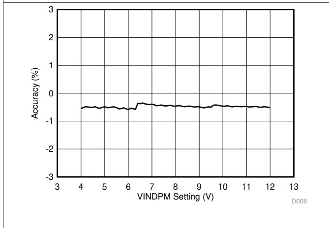
图 11. Input Voltage Limit Accuracy vs I 2 C VINDPM Setting
