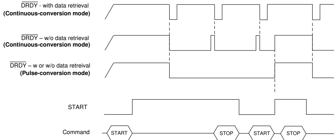
图 61. \overline{\text{DRDY}} Operation
