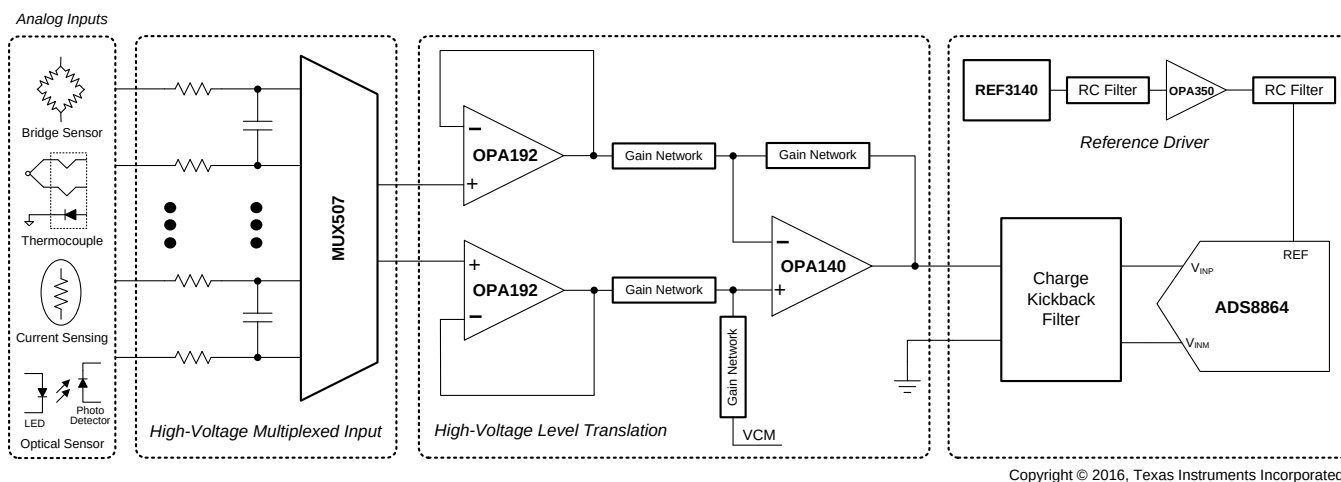
图 42. 16-Bit Precision Multiplexed Data-Acquisition System for High-Voltage Inputs With Lowest Distortion
