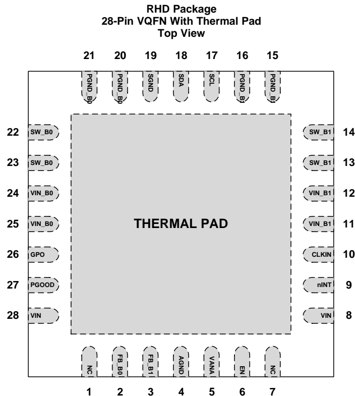
Pin Functions
