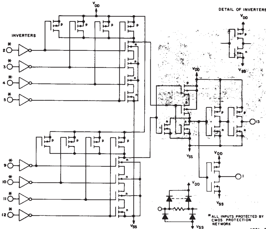
Fig. 8 - Schematic diagram.
