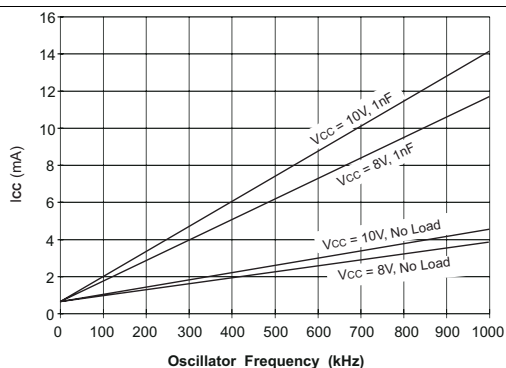
Figure 7. UCC2800-Q1 I_{CC} vs Oscillator Frequency
