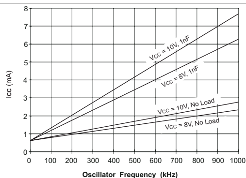
Figure 8. UCC2805-Q1 I_{CC} vs Oscillator Frequency
