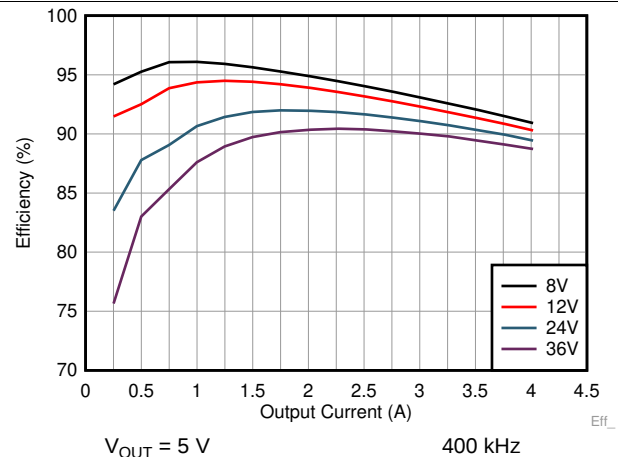
图 12. High-Load Efficiency
