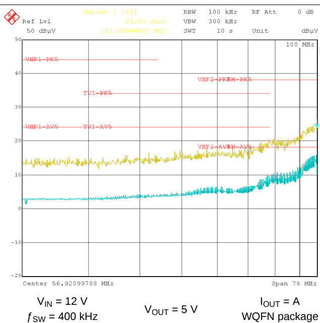
图 19. High Frequency Conducted EMI
