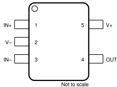
TLV9151 DCK Package (1) 5-Pin SC70 Top View
