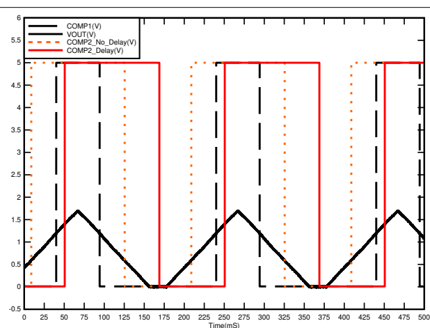
图 8-3. Polyswitch Warning and Fault Detection Circuit With Delay Response
