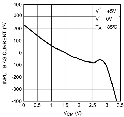
Figure 3. Input Bias Current vs. V_{CM}
