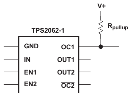
Figure 24. Typical Circuit for the \overline{\text{OC}} Pin
