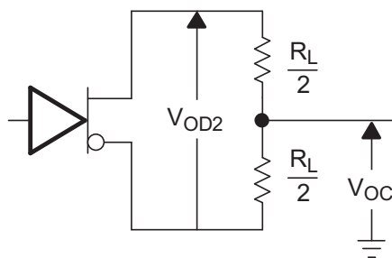
Figure 1. Driver Test Circuit, V_{OD} and V_{OC}
