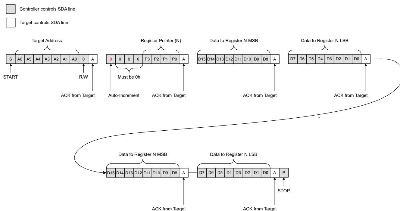
图 8-11. Repeated Write to Single Register
