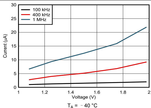
图 7-7. Supply Current vs. V_{DD} With Toggling SCL
