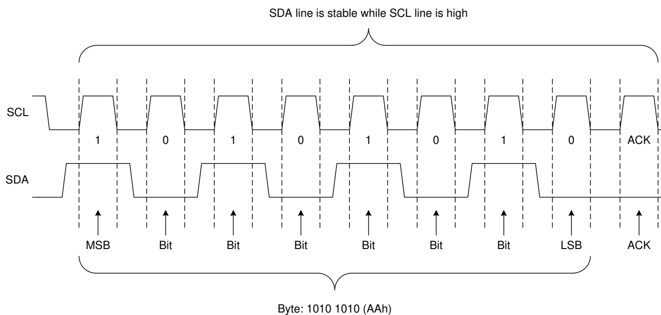
图 8-8. Bit Transfer
