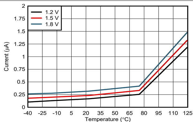
图 7-4. Active Current vs. Temperature
