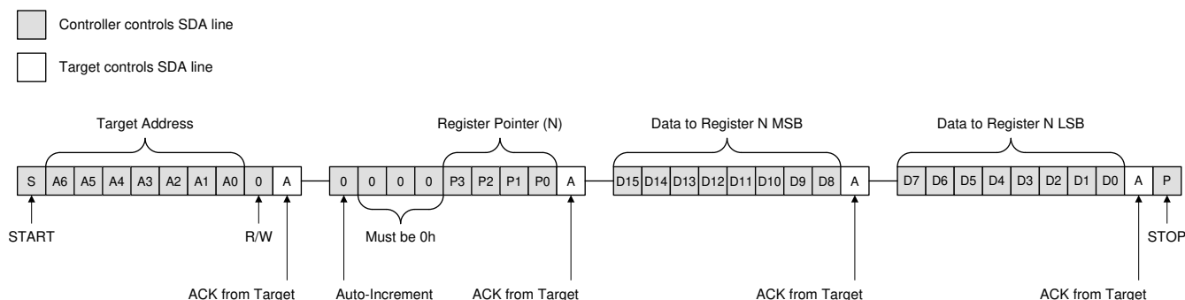
图 8-10. Write to Single Register
