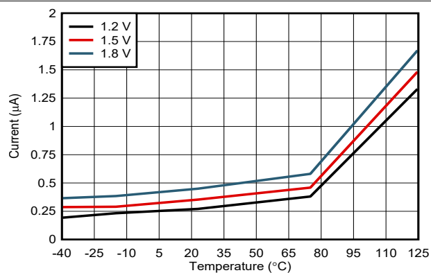
图 7-5. Standby Current vs. Temperature
