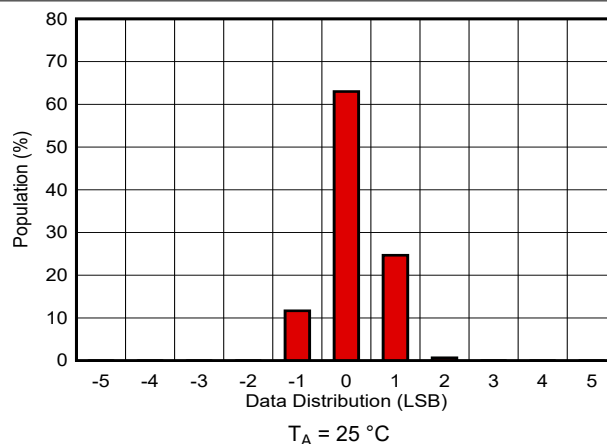
图 7-15. Data Distribution With 3.5-ms Conversion Time and Averaging On
