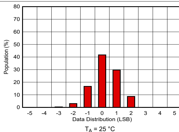
图 7-19. Data Distribution With 1.2-ms Conversion Time and Averaging On
