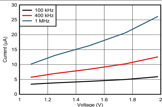
图 7-9. Supply Current vs. V_{DD} With Toggling SCL
