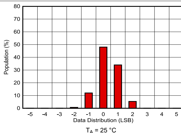
图 7-17. Data Distribution With 2-ms Conversion Time and Averaging On
