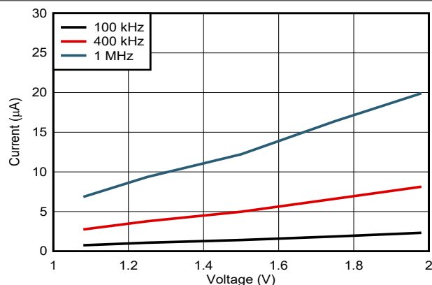
图 7-8. Supply Current vs. V_{DD} With Toggling SCL
