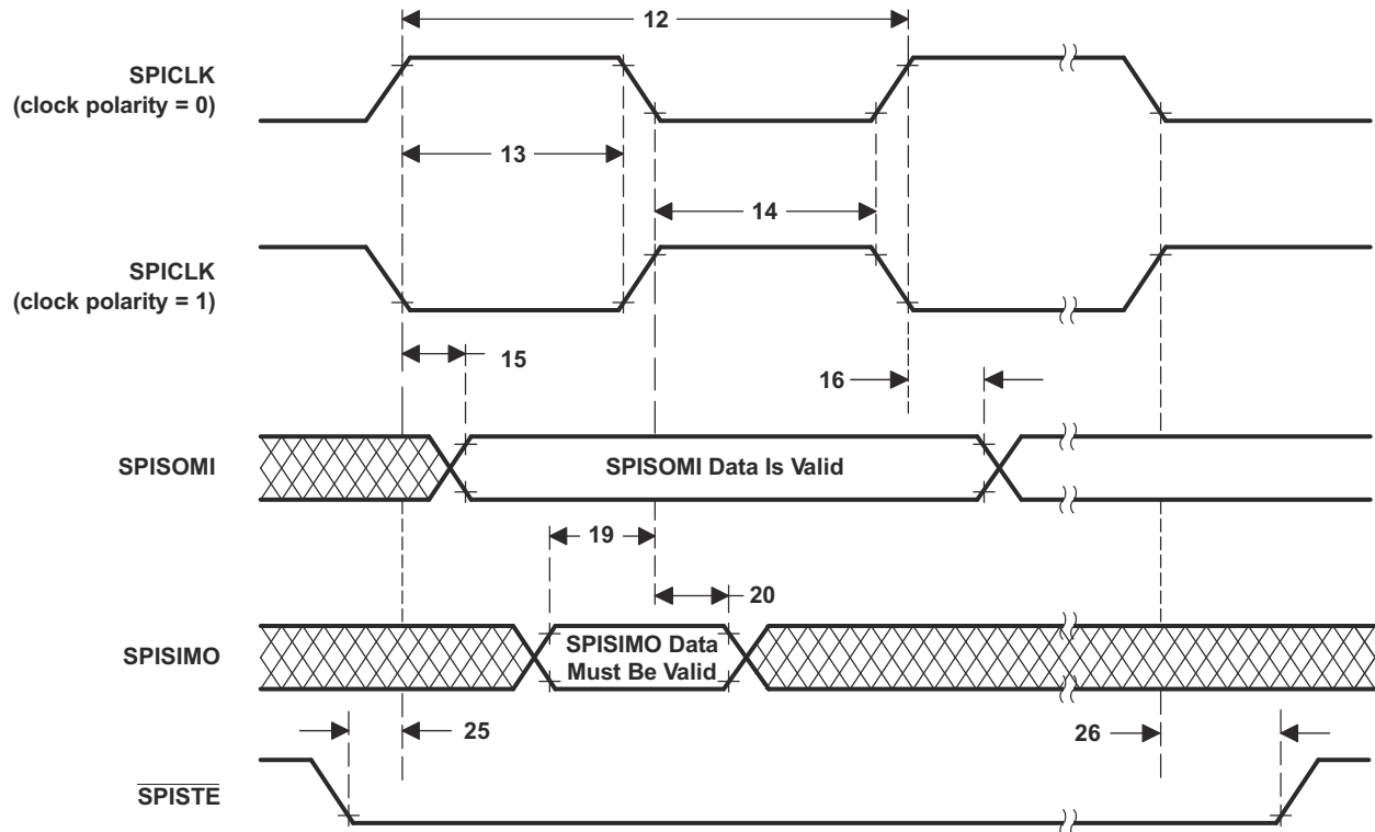
图 7-81. High-Speed SPI Slave Mode External Timing (Clock Phase = 0)
