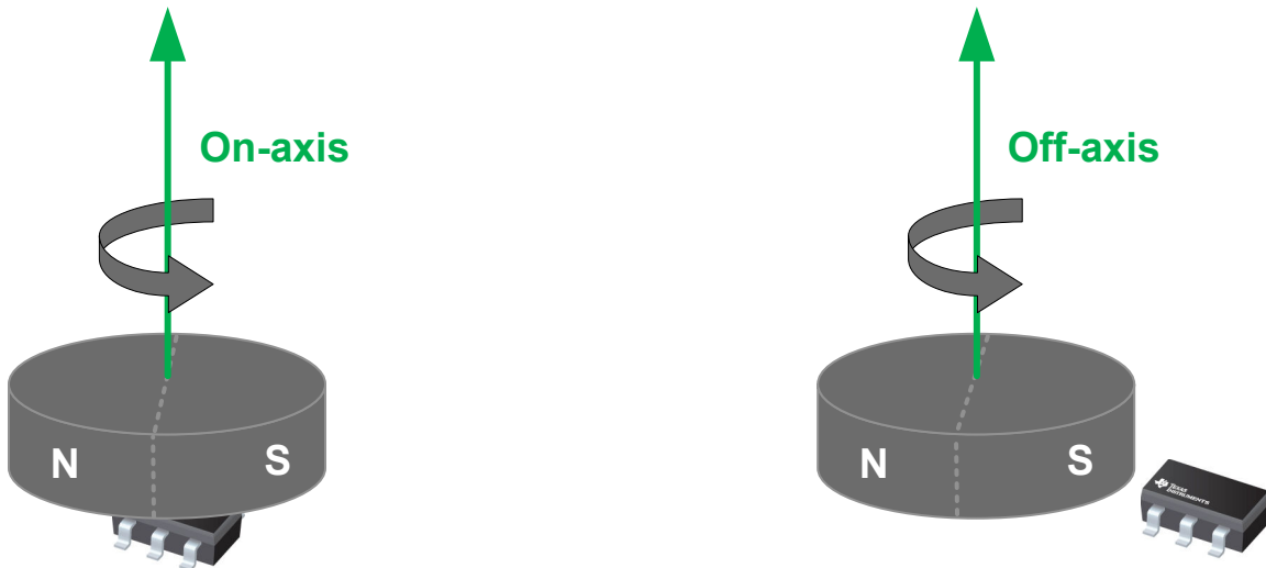
图 8-16. On-Axis vs. Off-Axis Angle Measurements
