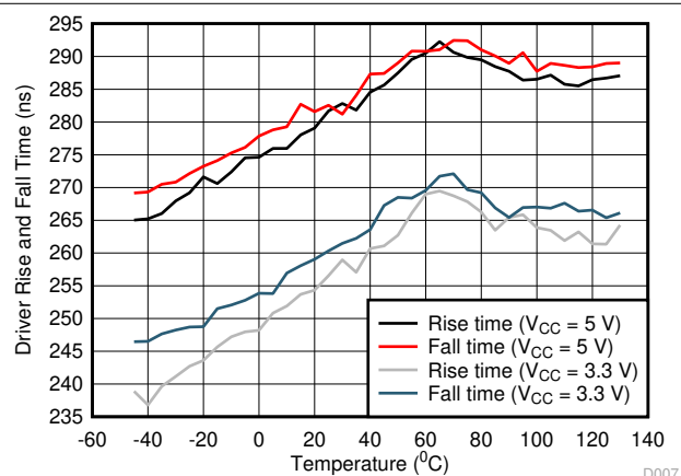
图 6-4. THVD2410 Driver Rise or Fall Time vs Temperature
