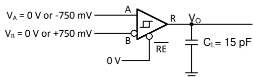
图 7-8. Measurement of Receiver Enable Times With Driver Disabled
