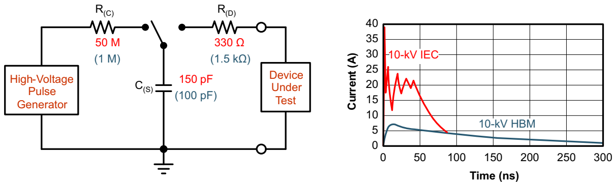
图 9-3. HBM and IEC ESD Models and Currents in Comparison (HBM Values in Parenthesis)
