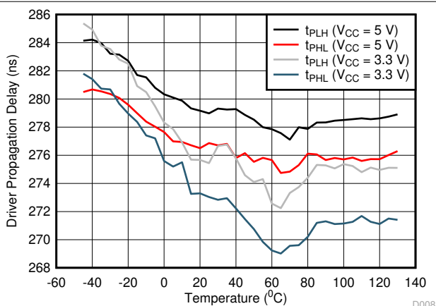
图 6-5. THVD2410 Driver Propagation Delay vs Temperature
