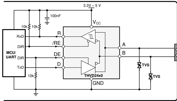
图 9-6. Transient Protection Against Surge Transients for Half-Duplex Devices
