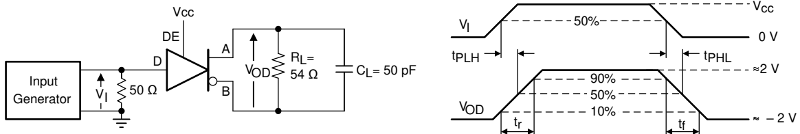
图 7-3. Measurement of Driver Differential Output Rise and Fall Times and Propagation Delays
