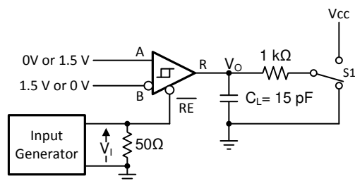
图 7-8. Measurement of Receiver Enable Times With Driver Disabled
