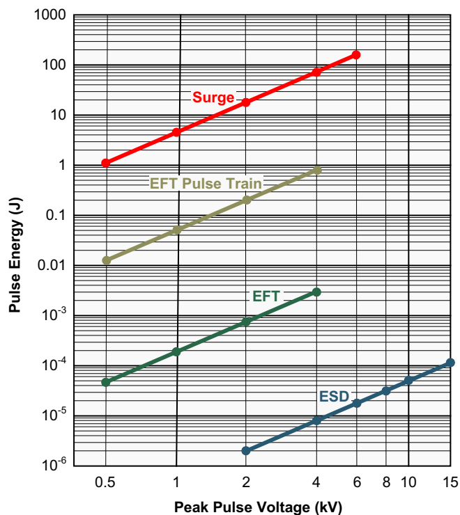
图 9-5. Comparison of Transient Energies
