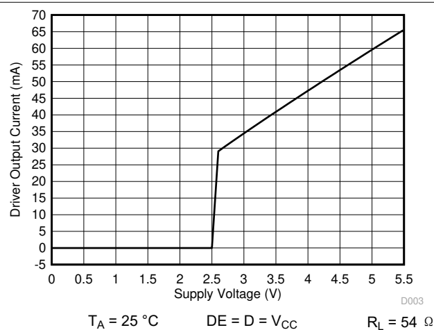
图 6-3. Driver Output Current vs Supply Voltage
