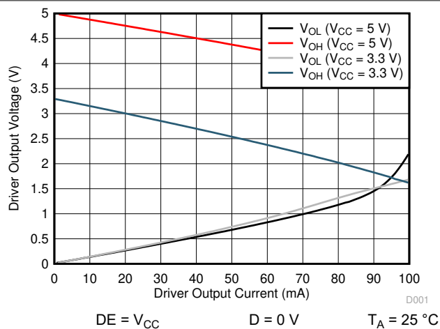
图 6-1. Driver Output Voltage vs Driver Output Current
