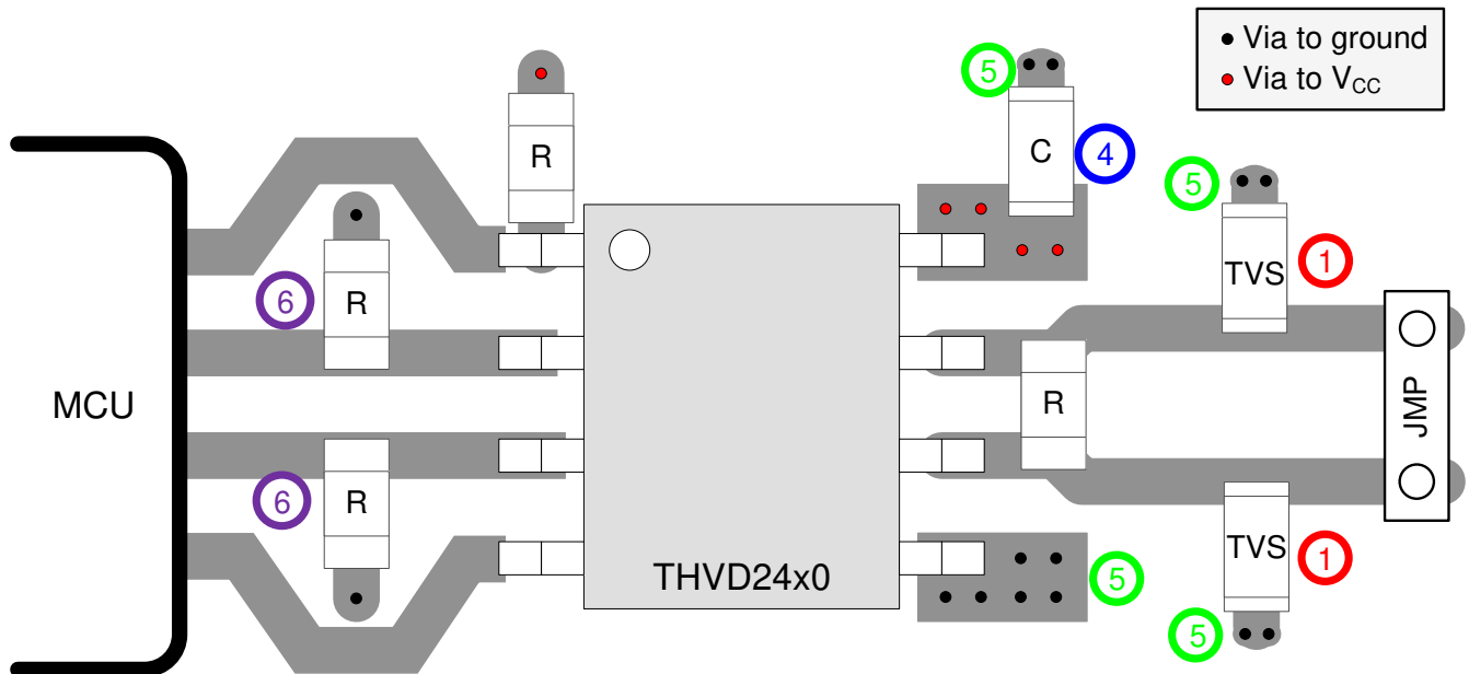
图 11-1. Half-Duplex Layout Example
