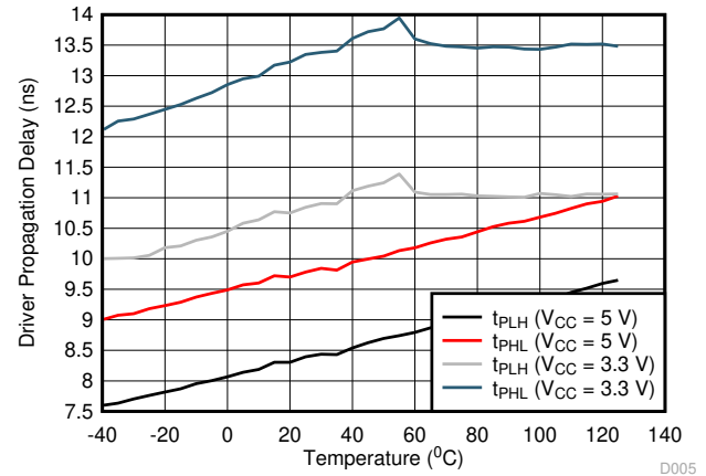
图 6-8. THVD2450 Driver Propagation Delay vs Temperature
