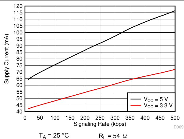
图 6-6. THVD2410 Supply Current vs Signal Rate
