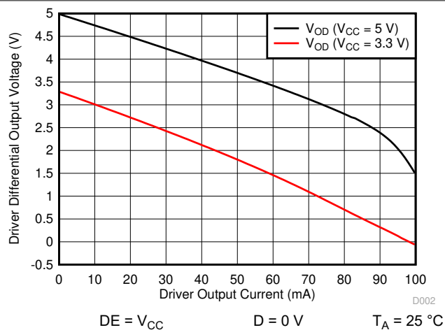
图 6-2. Driver Differential Output voltage vs Driver Output Current
