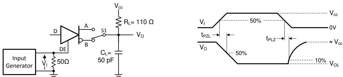
图 7-4. Measurement of Driver Enable and Disable Times With Active High Output and Pull-Down Load
