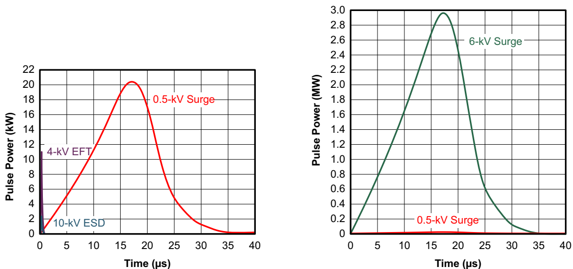
图 9-4. Power Comparison of ESD, EFT, and Surge Transients
