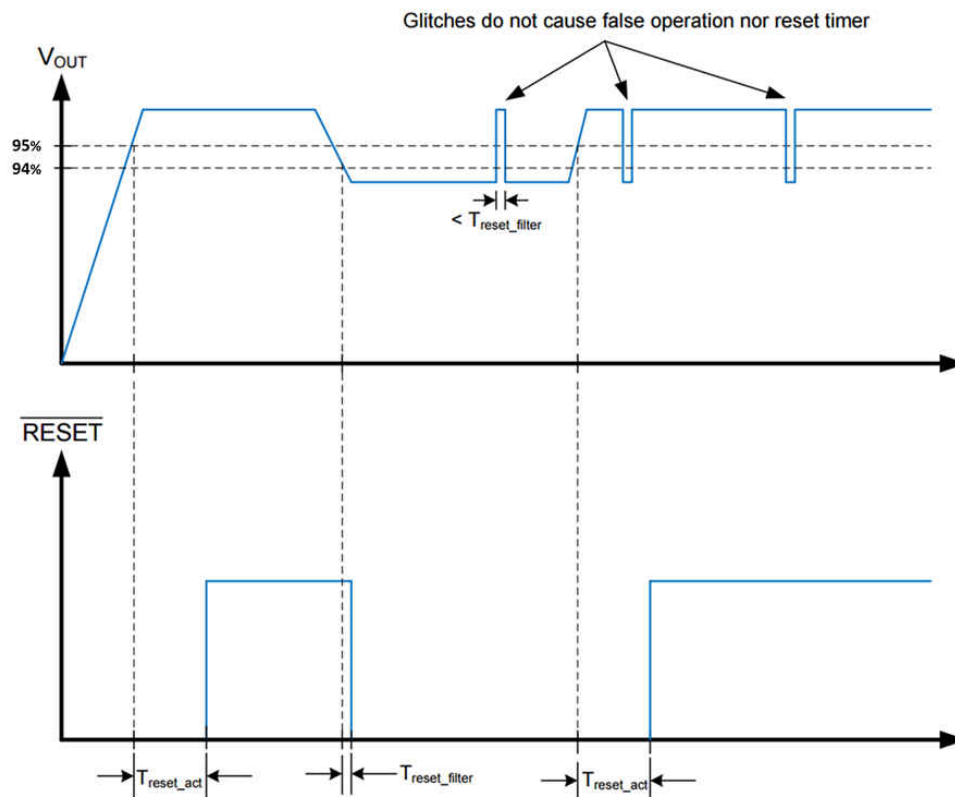
图 8-3. RESET Timing Behavior
