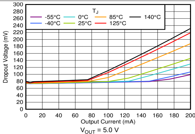
图 33. Dropout vs I_{OUT} and Temperature
