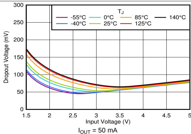
图 35. Dropout vs V_{IN} and Temperature
