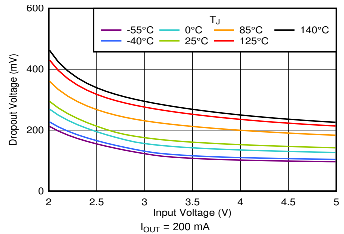
图 34. Dropout vs V_{IN} and Temperature
