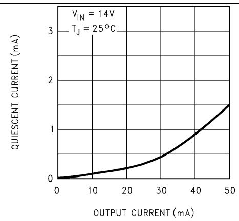
Figure 6. Quiescent Current
