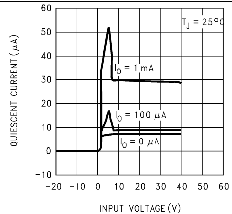
Figure 4. Quiescent Current
