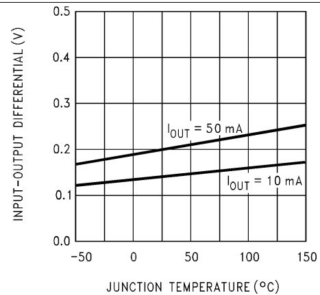
Figure 2. Dropout Voltage
