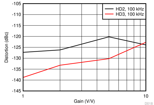
图 6-18. Harmonic Distortion vs Gain
