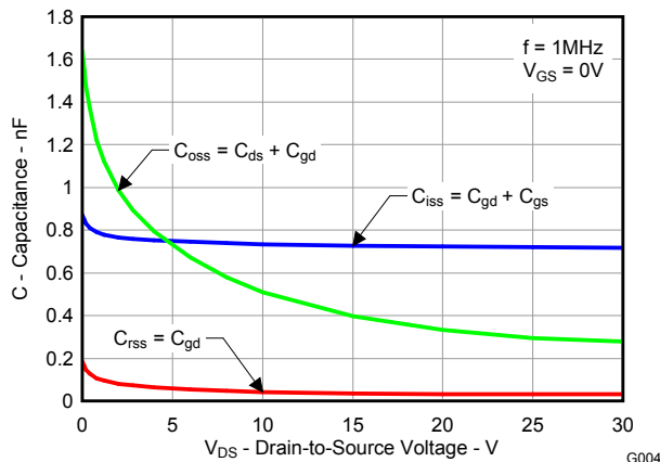
Figure 6. Capacitance
