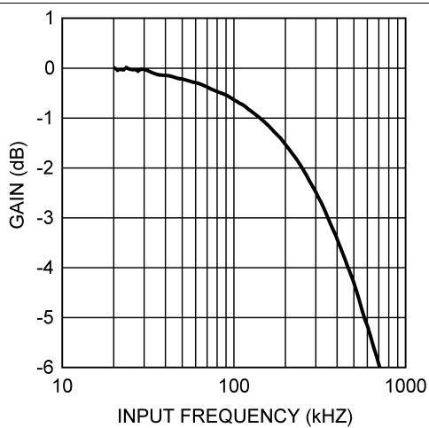
Figure 26. Multiplying Bandwidth
