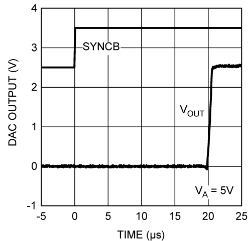
Figure 23. Wake-Up Time
