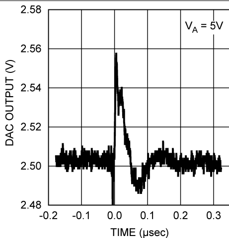
Figure 24. DAC-to-DAC Crosstalk
