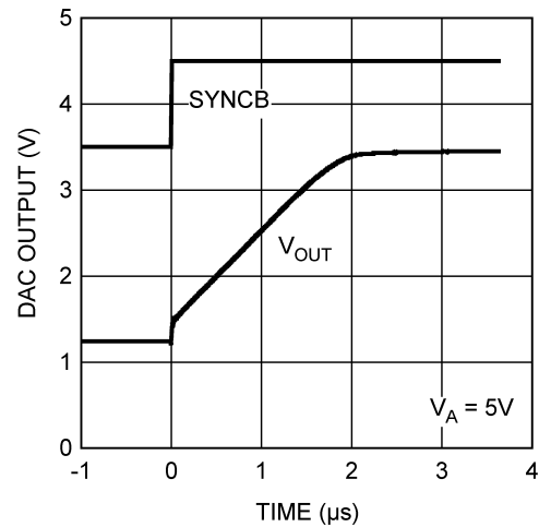
Figure 21. Settling Time
