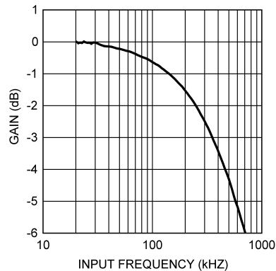
Figure 42. Multiplying Bandwidth
