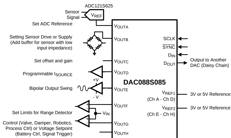
Figure 38. Industrial Application
