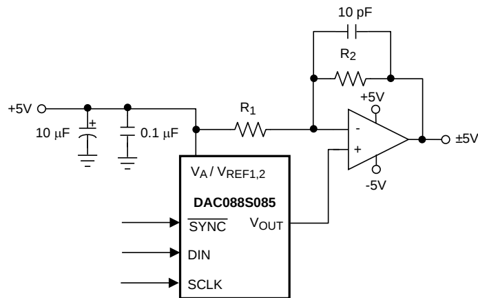
Figure 32. Bipolar Operation
