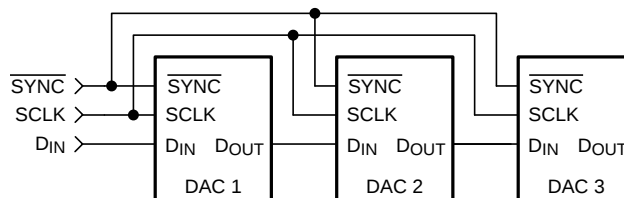
Figure 30. Daisy Chain Configuration
