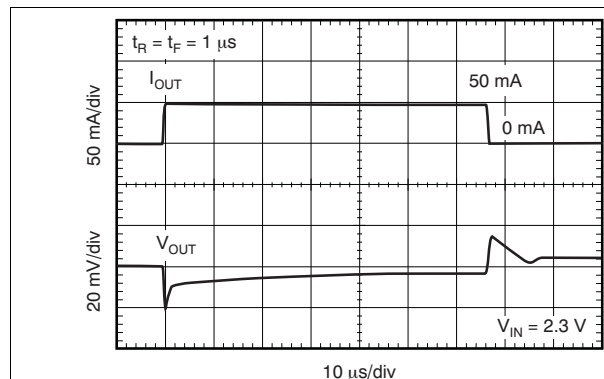
Figure 22. TLV70018 Load Transient Response
