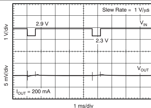
Figure 23. TLV70018 Line Transient Response
