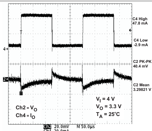
Figure 25. LDO2 Load Transient Response
