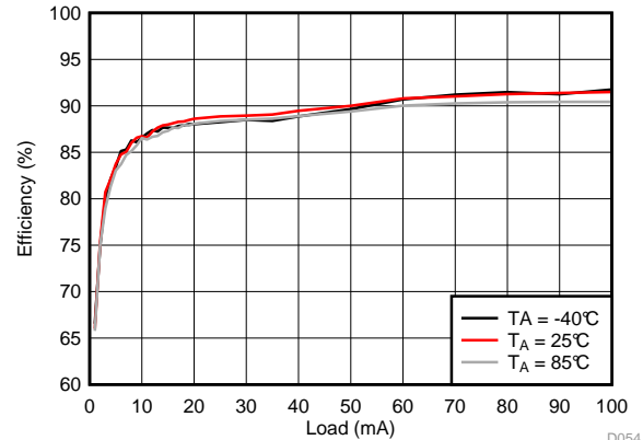
Figure 72. LCM Boost Efficiency
