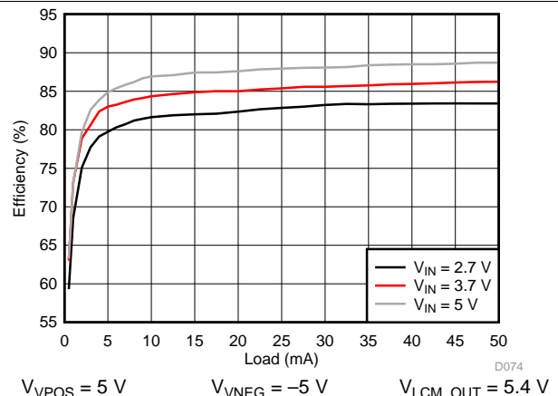
Figure 92. VPOS/VNEG Efficiency
