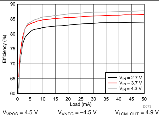
Figure 91. VPOS/VNEG Efficiency
