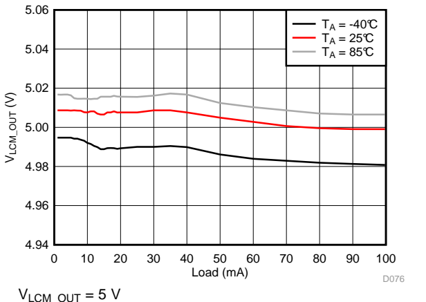
Figure 94. V_{LCM\_OUT} Load Regulation
