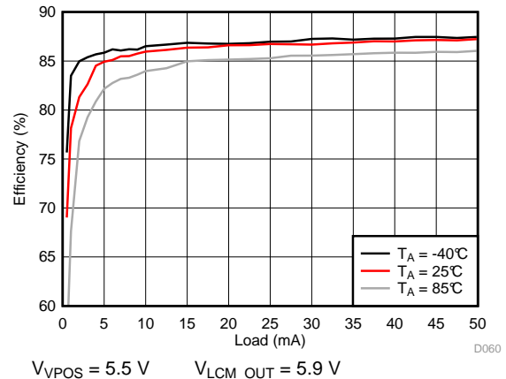
Figure 78. VPOS Efficiency
