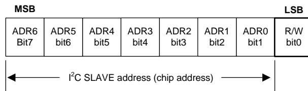
Figure 33. I 2 C Device Address
