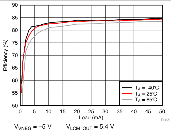
Figure 83. VNEG Efficiency
