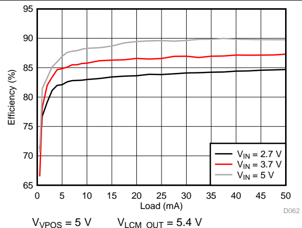
Figure 80. VPOS Efficiency
