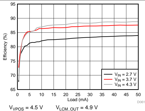
Figure 79. VPOS Efficiency
