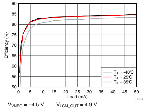
Figure 82. VNEG Efficiency
