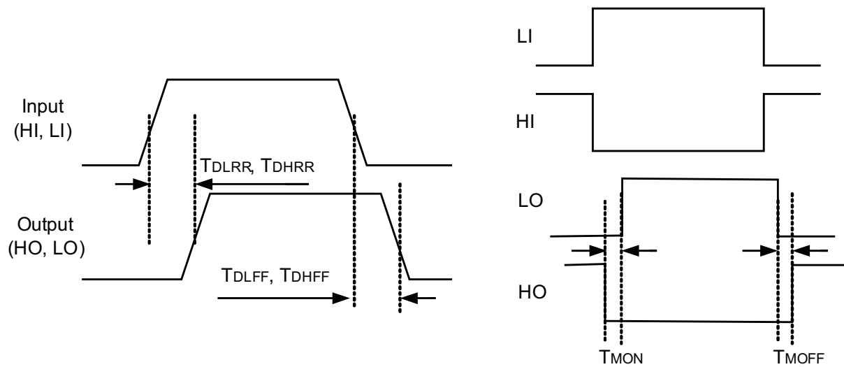
Figure 1. Timing Diagram
