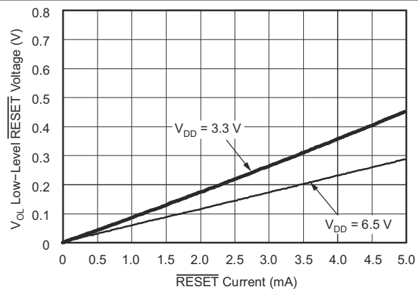
图 7-8. Low-Level \overline{RESET} Voltage vs \overline{RESET} Current
