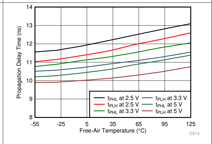
Figure 14. Propagation Delay Time vs Free-Air Temperature
