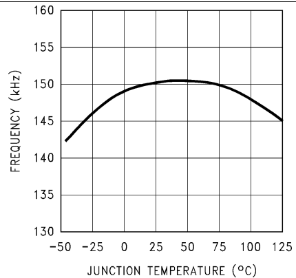
Figure 12. Switching Frequency
