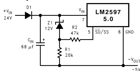
Figure 28. Undervoltage Lockout With Hysteresis for an Inverting Regulator
