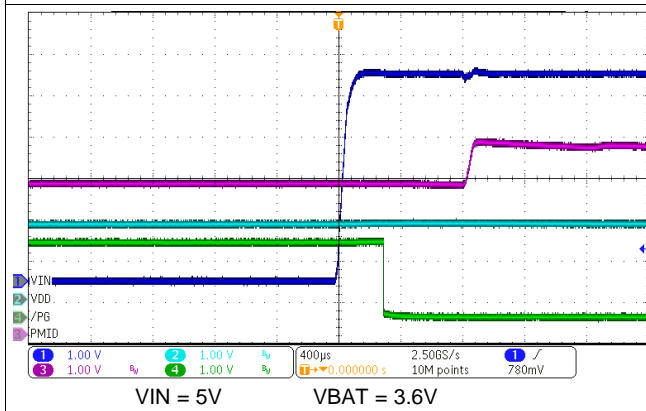
图 70. \overline{PG} Power Good Function - IN Supply Insertion
