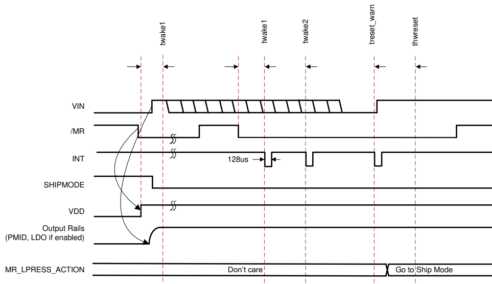
图 19. MR Wake from Ship Mode – VIN Dependencies
