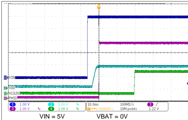
图 62. Power Up from IN Supply Insertion with No Battery
