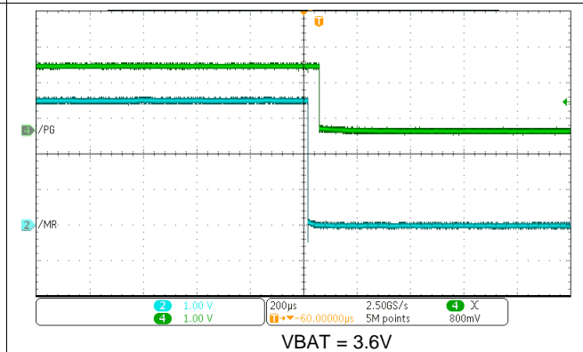
图 73. \overline{PG} \overline{MR} Level Shift Function - \overline{MR} Falling
