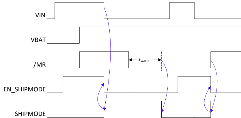
图 28. Ship Mode Entry Based On EN_SHIPMODE bit
