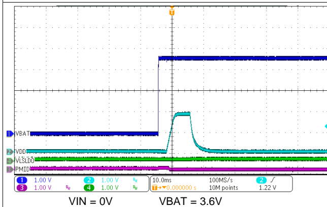
图 64. Wake In To Ship Mode on Battery Insertion with No IN Supply
