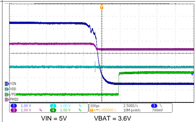
图 71. \overline{PG} Power Good Function - IN Supply Removal
