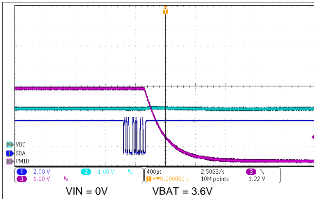
图 68. HW Reset Through I 2 C Command
