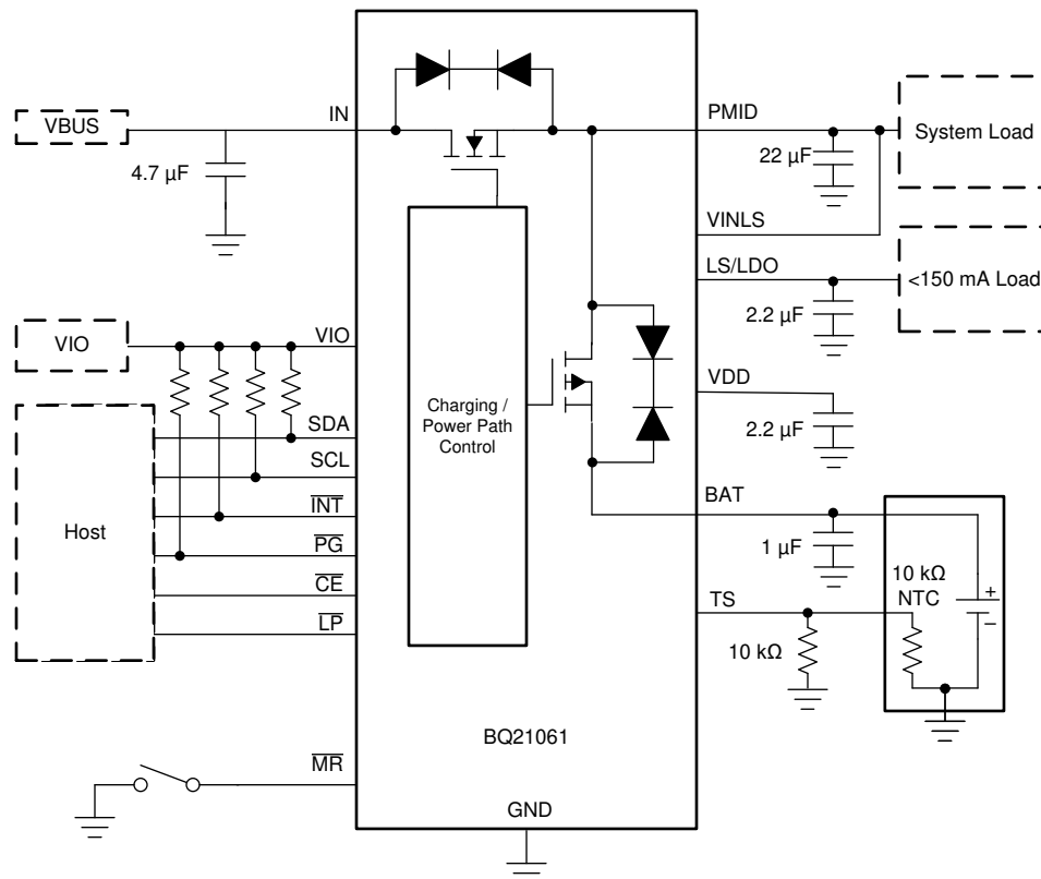
图 61. Typical Application Diagram
