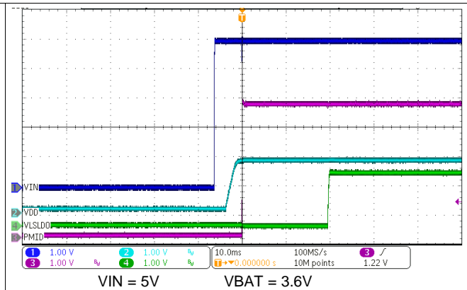
图 63. Power Up from Ship Mode with IN Supply Insertion
