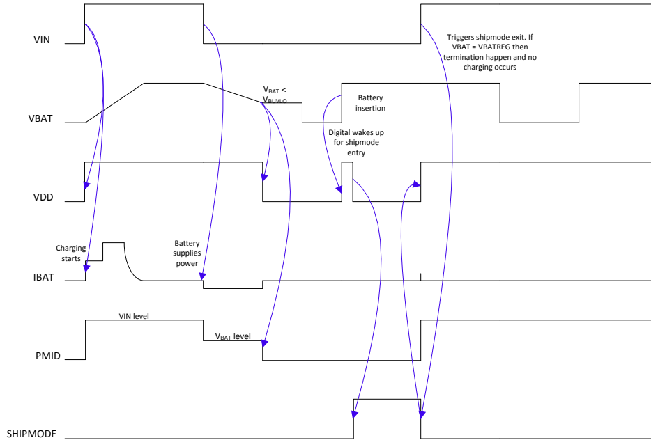
图 29. BQ21061 Wake-Up Upon Supply Insertion
