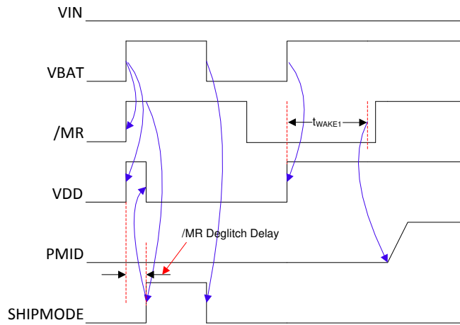
图 30. BQ21061 Wake-Up Upon Battery Insertion
