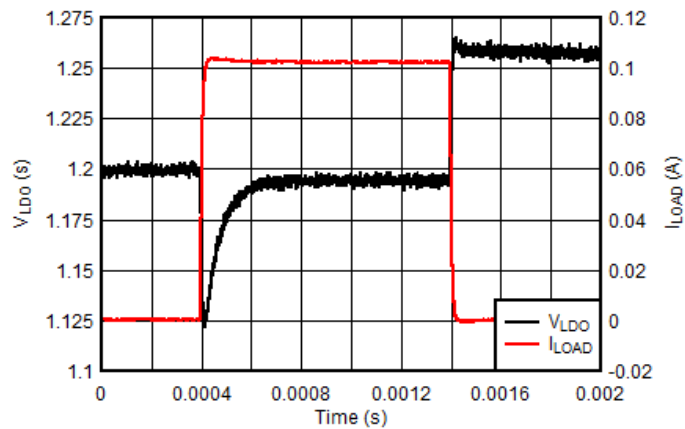
图 80. LDO Load Transient - VLDO = 1.2V
