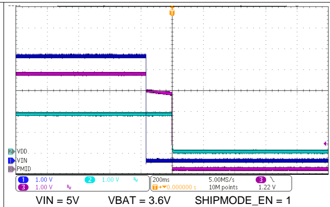
图 69. Ship Mode Entry on IN Supply Removal
