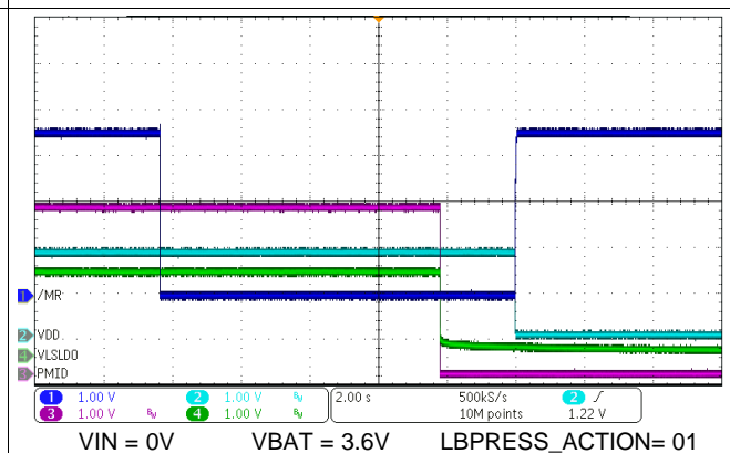
图 67. Ship Mode Entry with \overline{MR} Long Button Press
