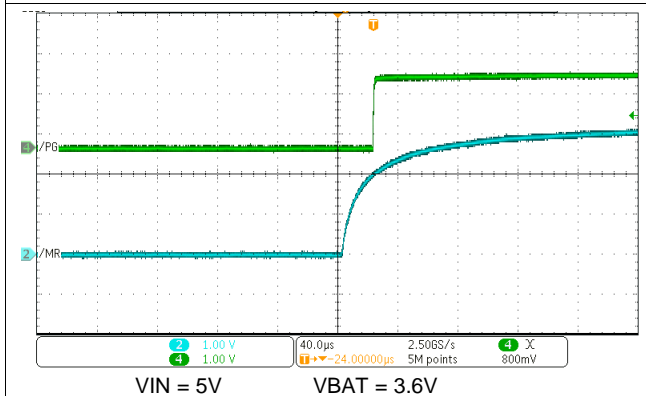
图 72. \overline{PG} \overline{MR} Level Shift Function - \overline{MR} Rising
