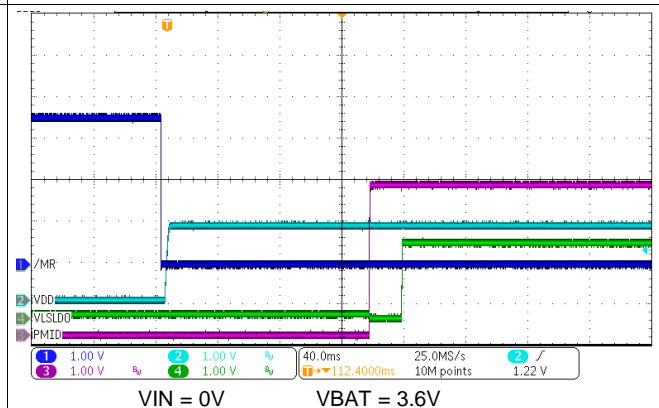
图 65. Power Up from Ship Mode with \overline{MR} Press
