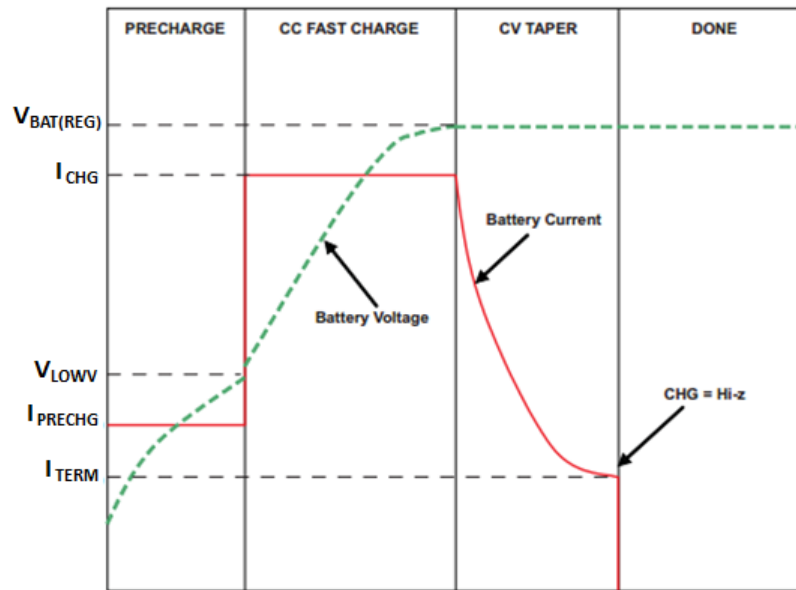
图 17. BQ21061 Typical Charge Cycle
