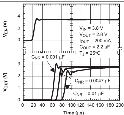
Figure 19. TPS73028 Output Voltage, Enable Voltage vs Time (Start-Up)
