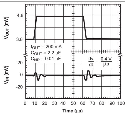
Figure 20. TPS73028 Line Transient Response
