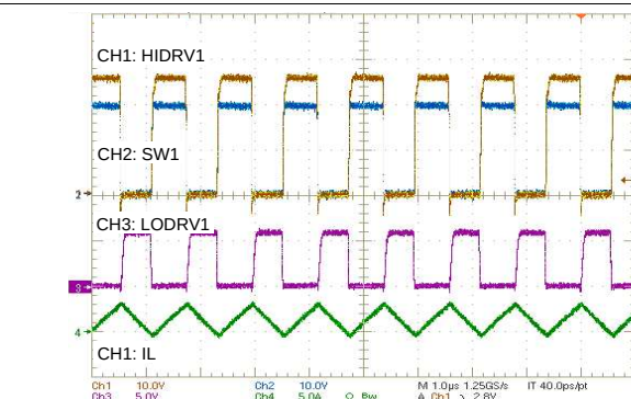
Figure 39. System Regulation
