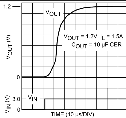
Figure 21. Turnon Time
