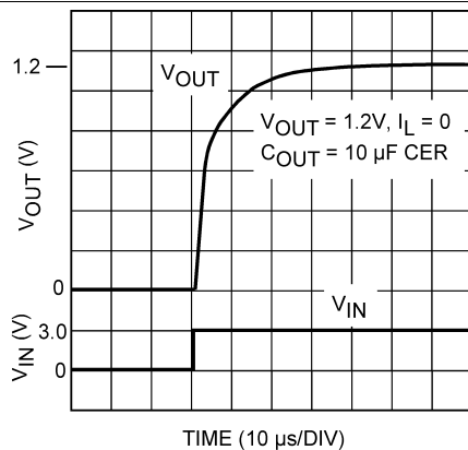
Figure 20. Turnon Time
