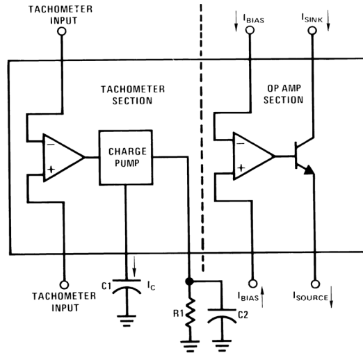
Figure 13. Test Circuit
