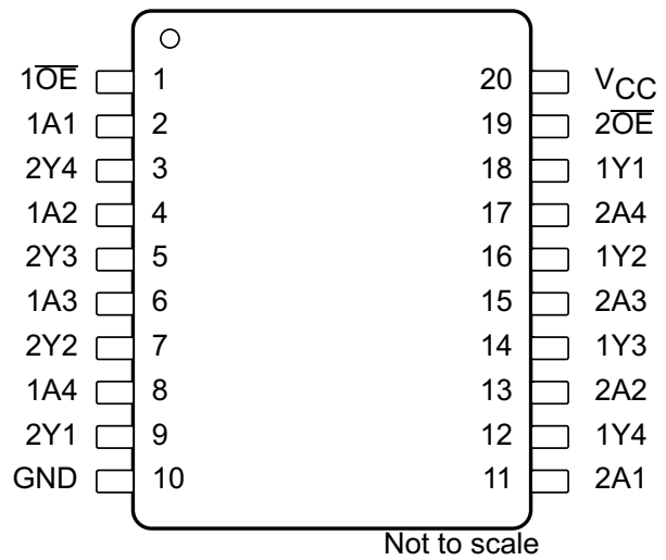
图 5-2. DB, DGV, DW, N, NS, and PW Packages 20-Pin SSOP, TVSOP, SOIC, PDIP, SO, and TSSOP Front View
