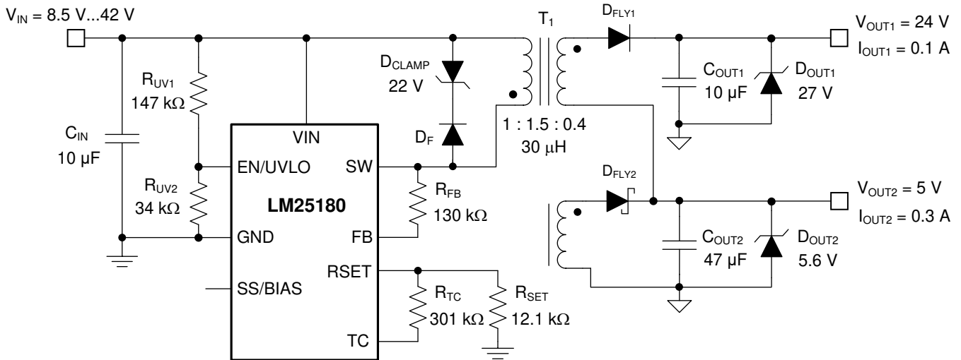
图 45. Schematic for Design 3 With V_{IN(nom)} = 24 V, V_{OUT1} = 24 V, V_{OUT2} = 5 V
